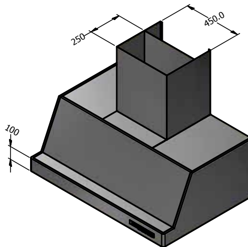
Top Ducted
