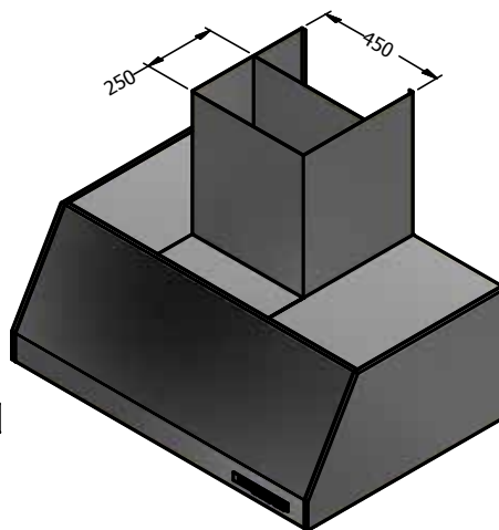
Top Ducted
