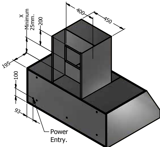
Back Ducted
