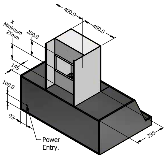
Back Ducted
